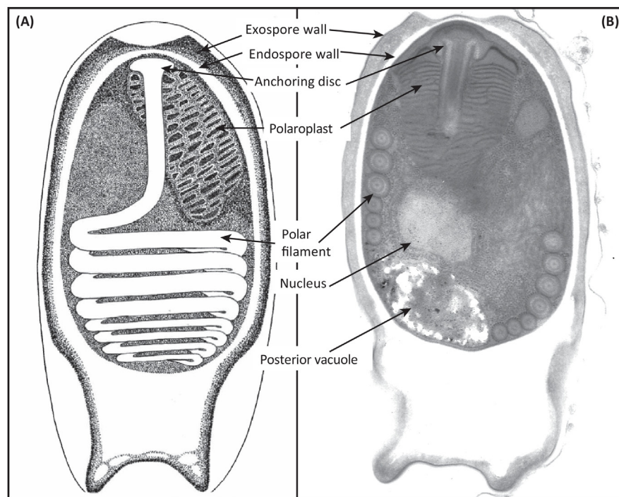
Figure 1. The Features of a Typical Microsporidian Spore. (A) Diagram. (B) Transmission electron micrograph. The rigid spore wall is composed of the exospores, the endospore, and a sophisticated extrusion apparatus containing the polar filament, polaroplast, and the posterior vacuole.
