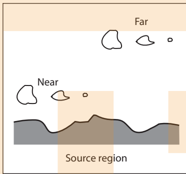
A. MacArthur & Wilson's Theory of Island Biogeography
