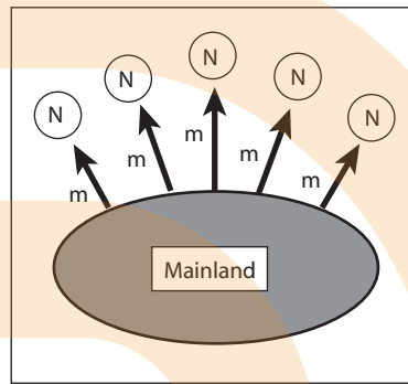
B. Wright's mainland-island model of population genetics
