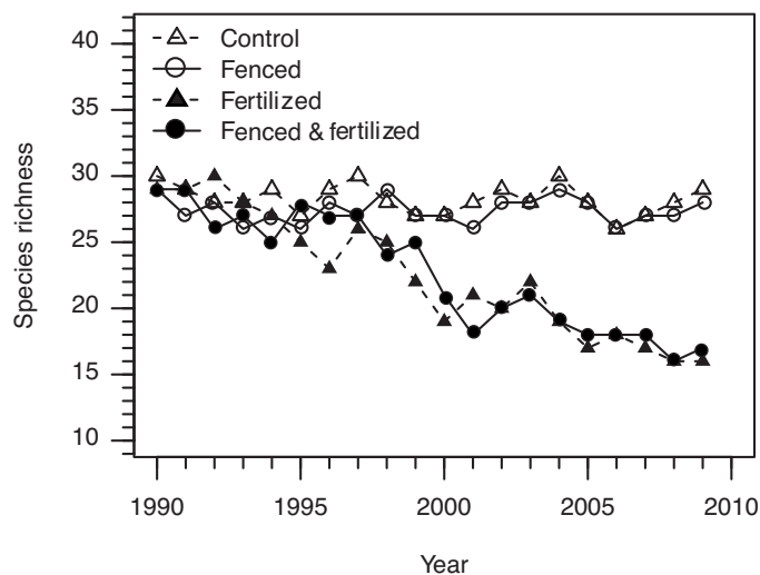
FIG. 1. Species richness (number of species) in plots subjected to fertilization and enclosure treatments from 1990 to 2009. Solid symbols are fertilized plots, and open symbols, unfertilized plots. Triangles with dashed lines are unfenced plots, and circles with solid lines are fenced plots. Based on Turkington et al. (2002).
