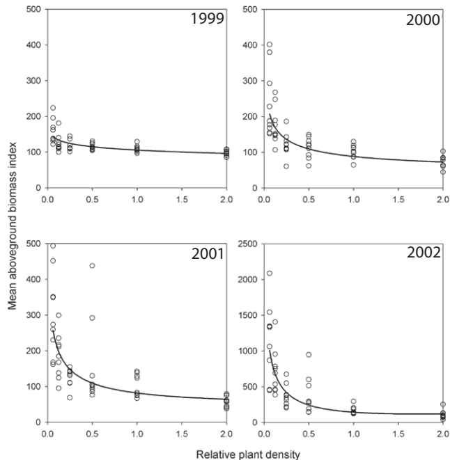
FIG. 4. The effect of initial community density on the mean aboveground plant biomass index (aboveground biomass (g) per plot divided by the community density) for 1999 to 2002. Best-fit lines shown are statistically significant ( p < 0.001 ). No significant slope would be expected in the absence of interactions, and a negative slope suggests negative density dependence or competition. Note that the scale for the Y-axis in 2002 is different than for other years. In all years, competition began to reduce mean plant size at 1/8 \times the natural community density ( 1 \times ). In 2001 and 2002, two and three years, respectively, after treatments were initiated, the community reached carrying capacity at approximately the natural density (M.A. Treberg and R. Turkington, unpubl. data).
