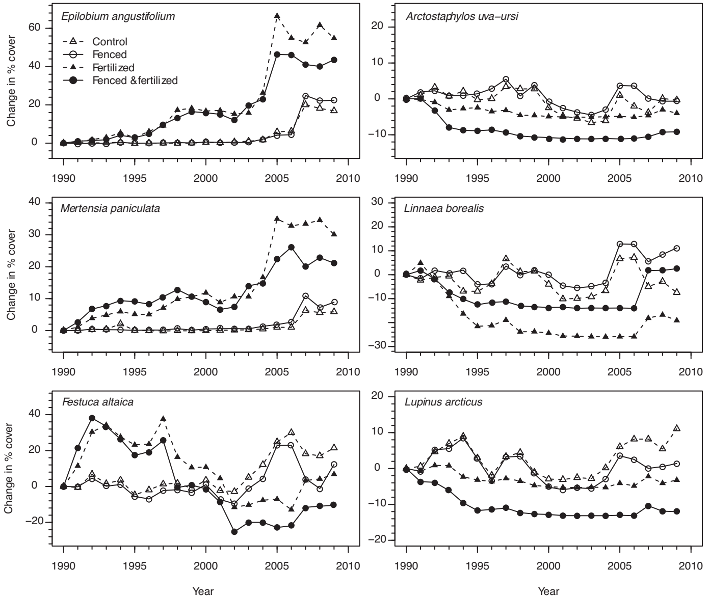
FIG. 2. Change in percent cover of six species, (left) three that initially increased and (right) three that initially decreased, in response to fertilization treatments from 1990 to 2009. Plots were treated from 1990 to 2009. Solid symbols are fertilized plots, and open symbols, unfertilized plots. Triangles with dashed lines are unfenced plots, and circles with solid lines are fenced plots. Error bars have been omitted for clarity. Based on Turkington et al. (2002).
